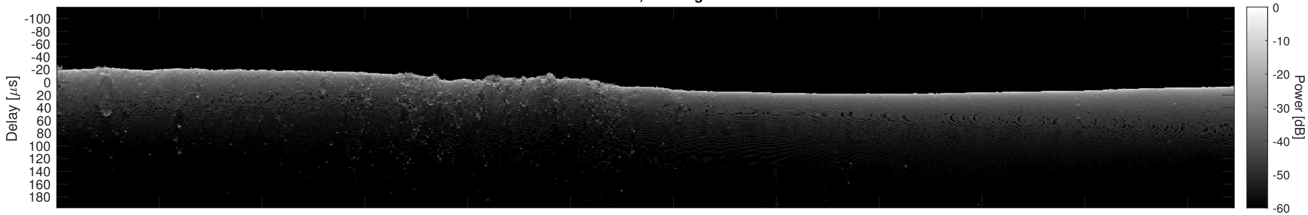
Orbit 16499, Cluttergram
