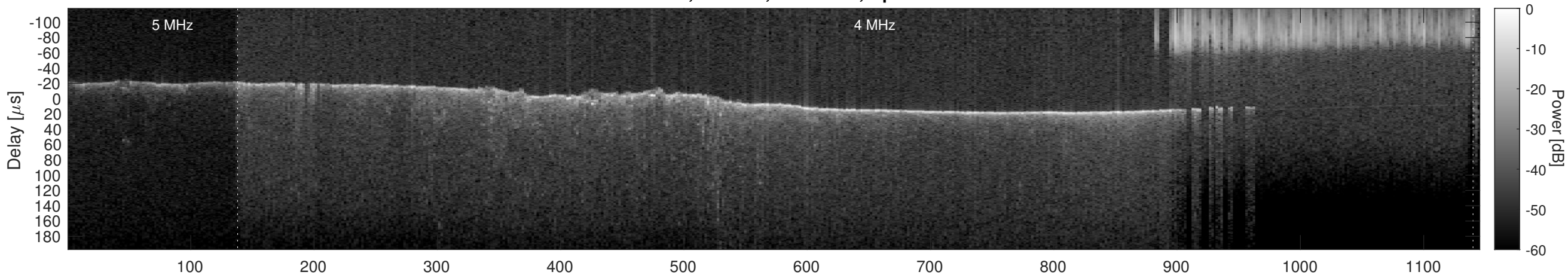
Orbit 16499, Cluttergram
