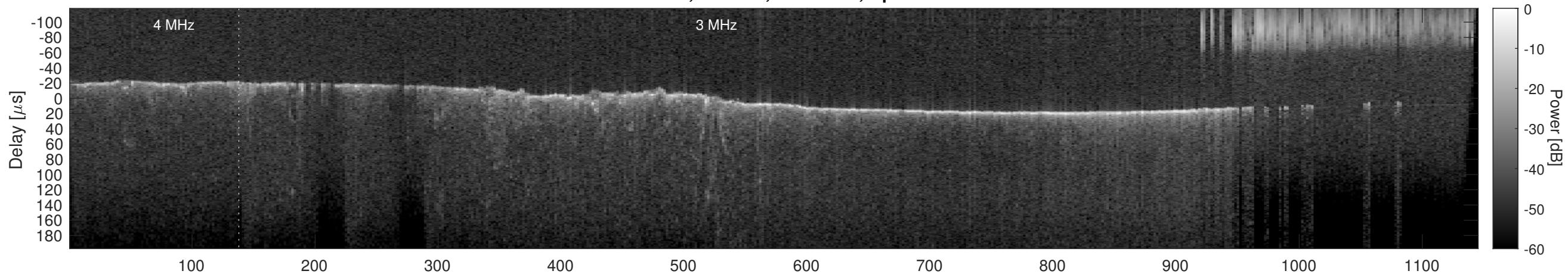
Orbit 16499, Cluttergram
