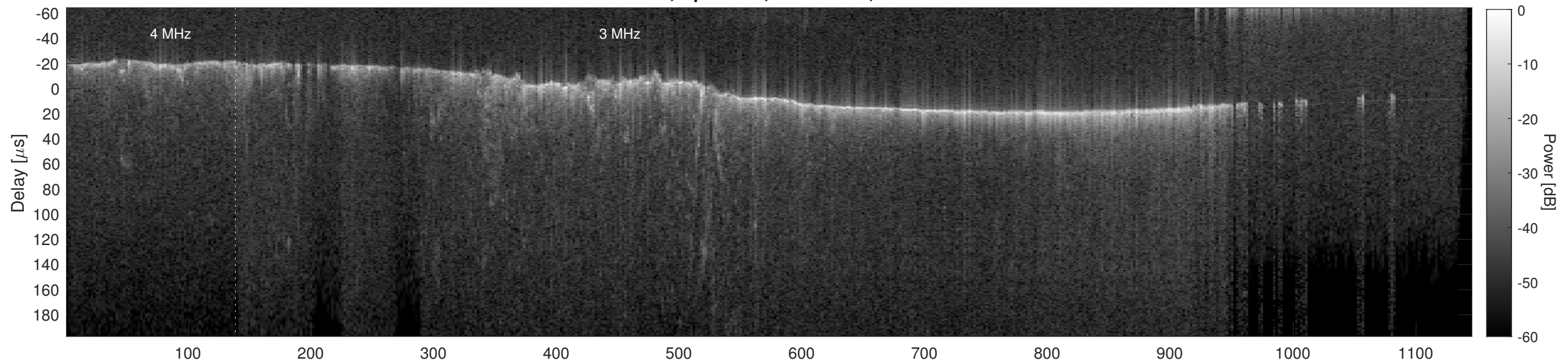
Orbit 16499, Cluttergram
