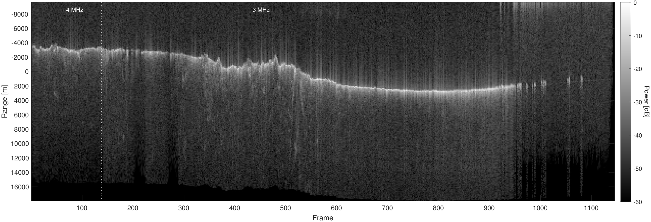
Orbit 16499, Optimized, No Window, Depth-Corrected, Channel 2
