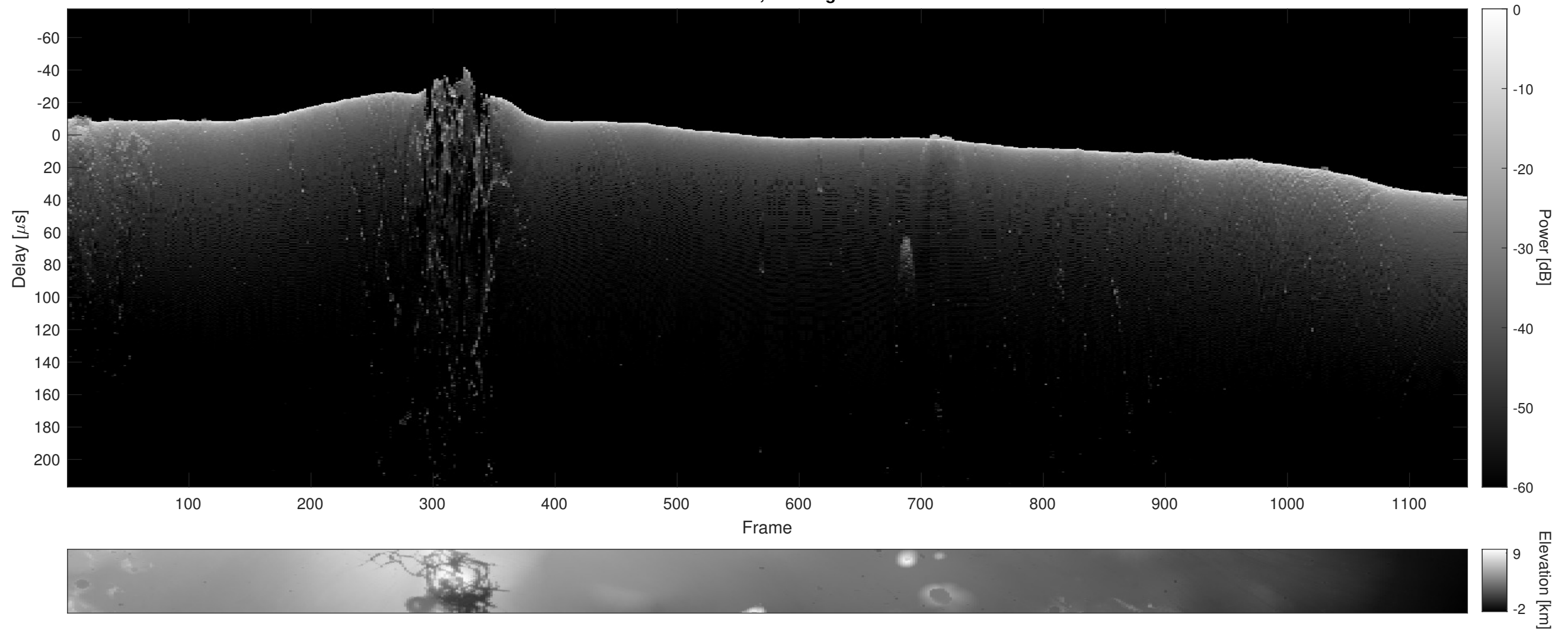
Orbit 16501, Cluttergram
