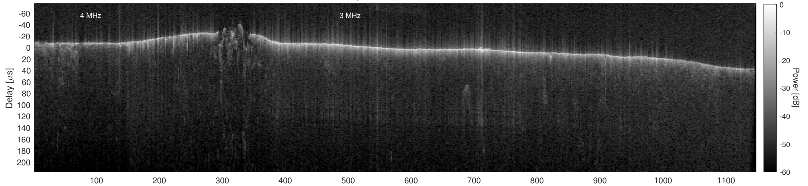
Orbit 16501, Cluttergram
