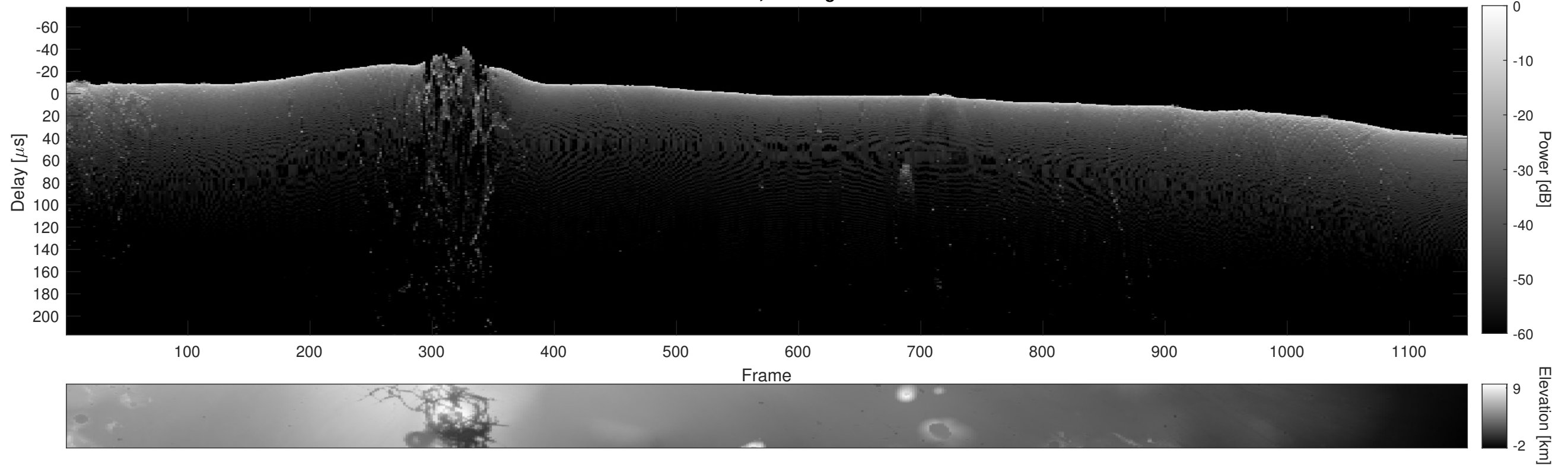
Orbit 16501, Cluttergram
