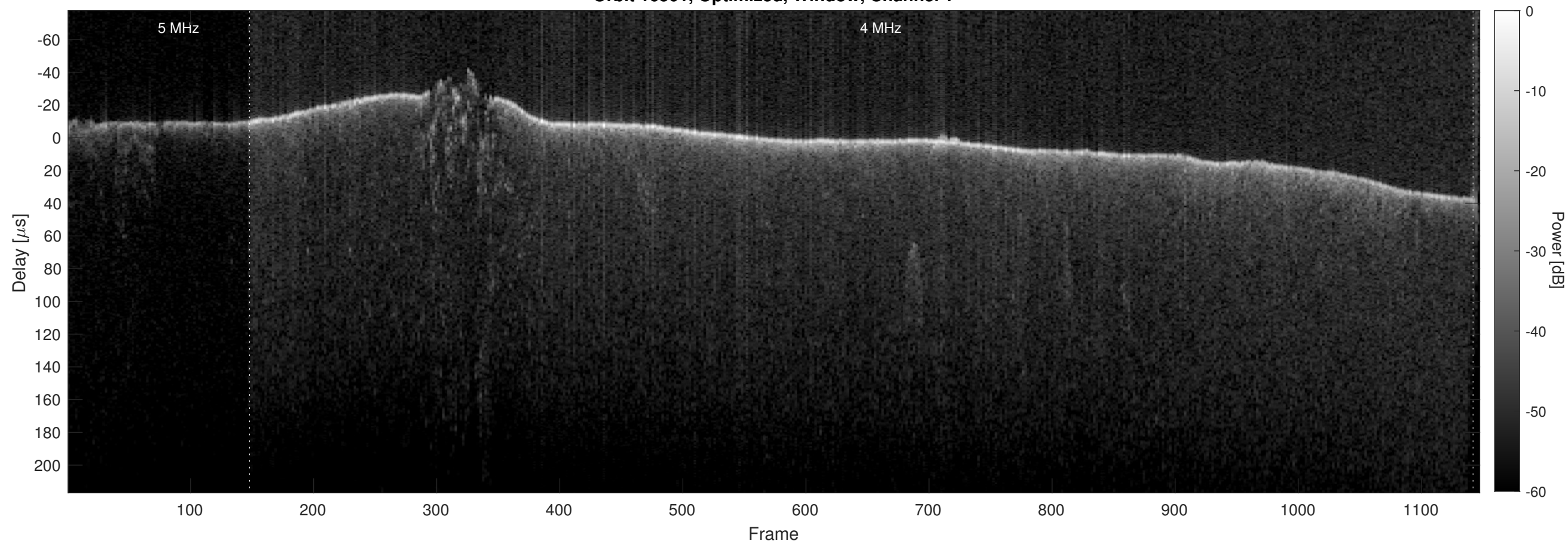
Orbit 16501, Optimized, Window, Channel 2
