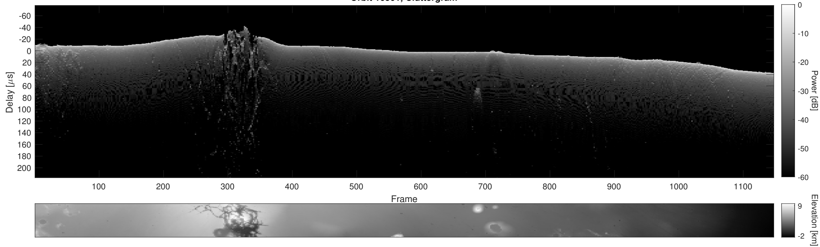
Orbit 16501, Cluttergram
