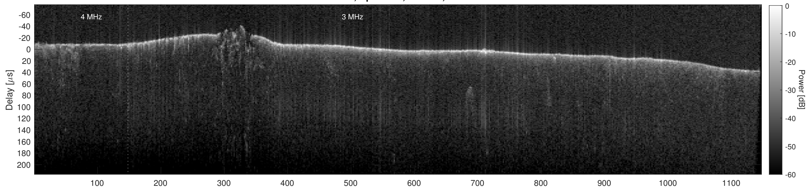
Orbit 16501, Cluttergram
