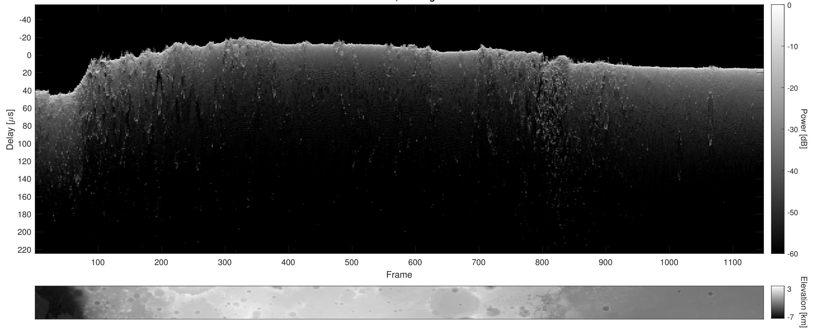
Orbit 16503, Cluttergram
