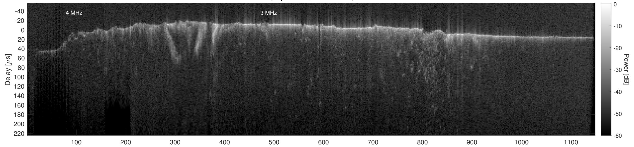
Orbit 16503, Cluttergram
