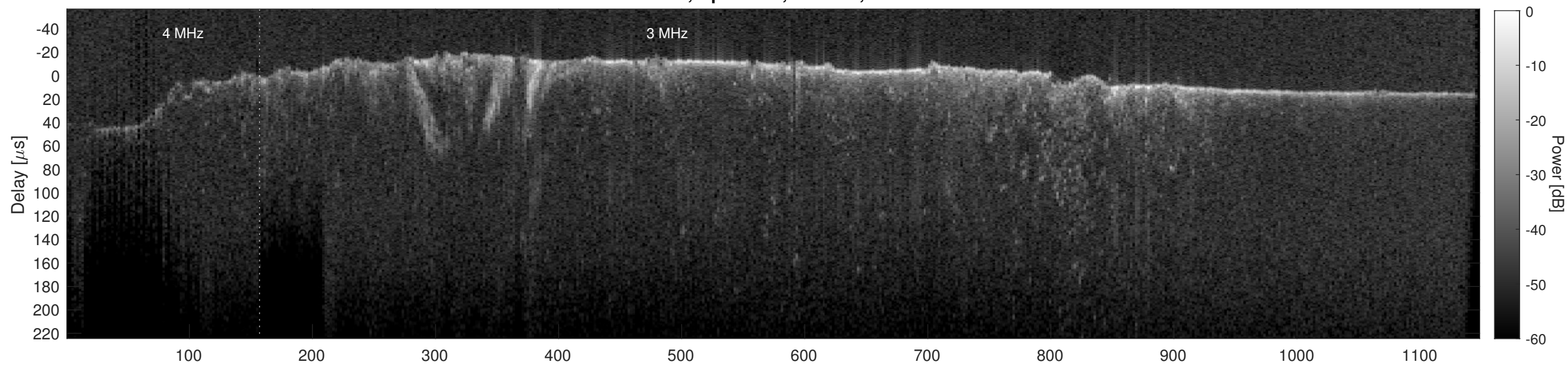
Orbit 16503, Cluttergram
