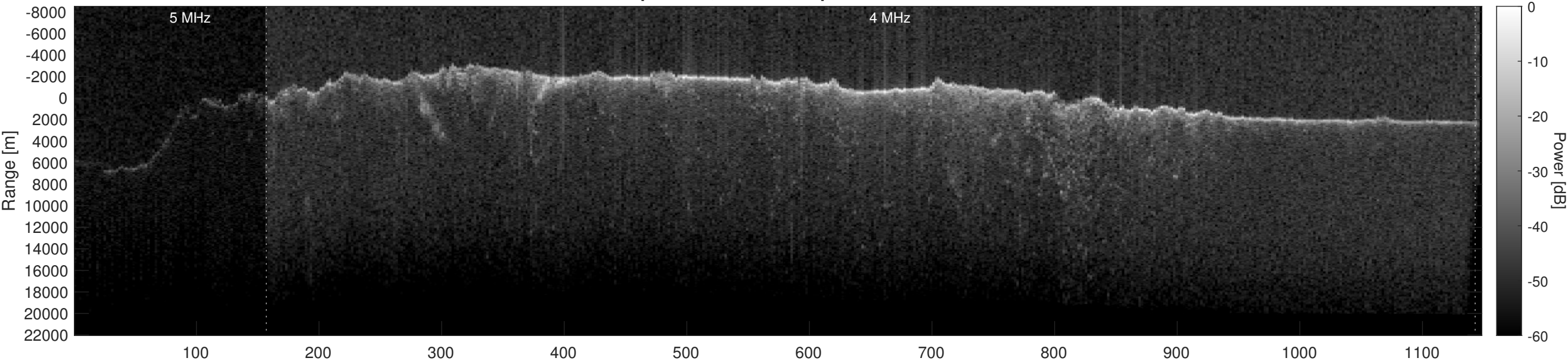
Orbit 16503, Optimized, Window, Depth-Corrected, Channel 2
