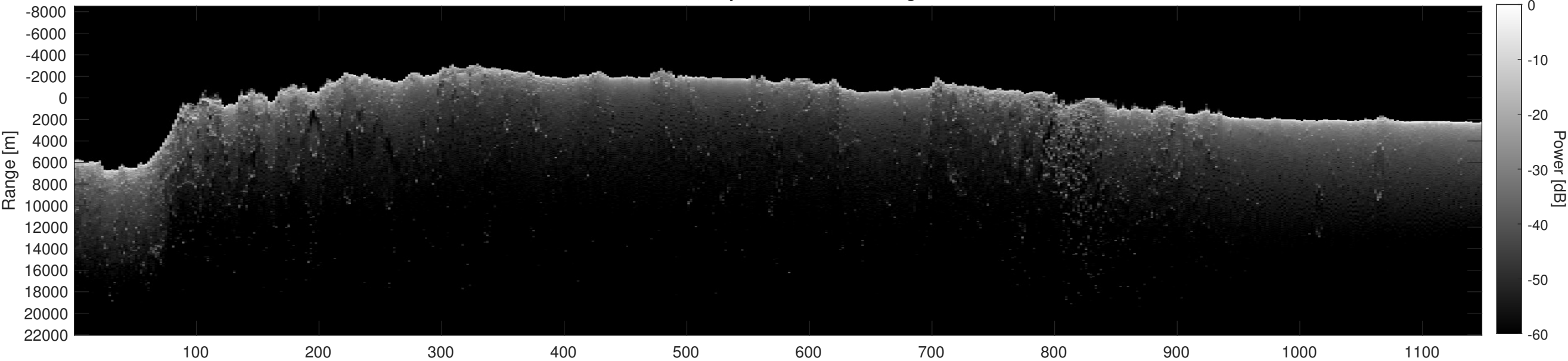
Orbit 16503, Depth-Corrected Cluttergram
