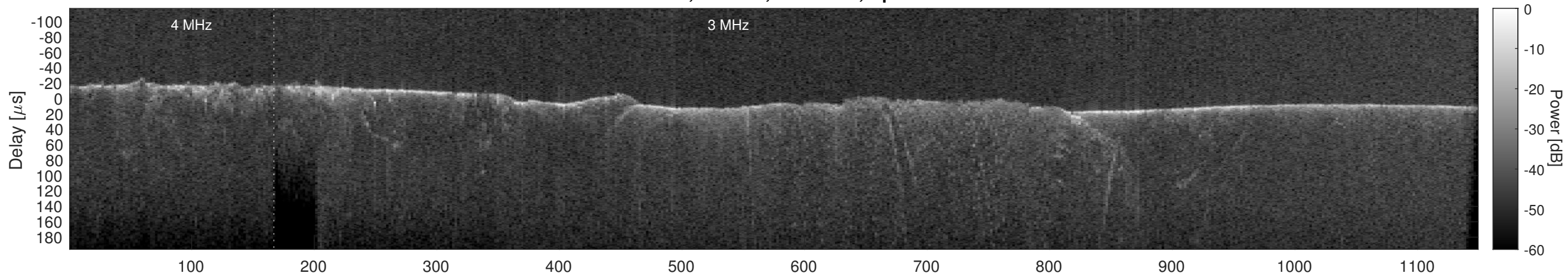
Orbit 16505, Cluttergram
