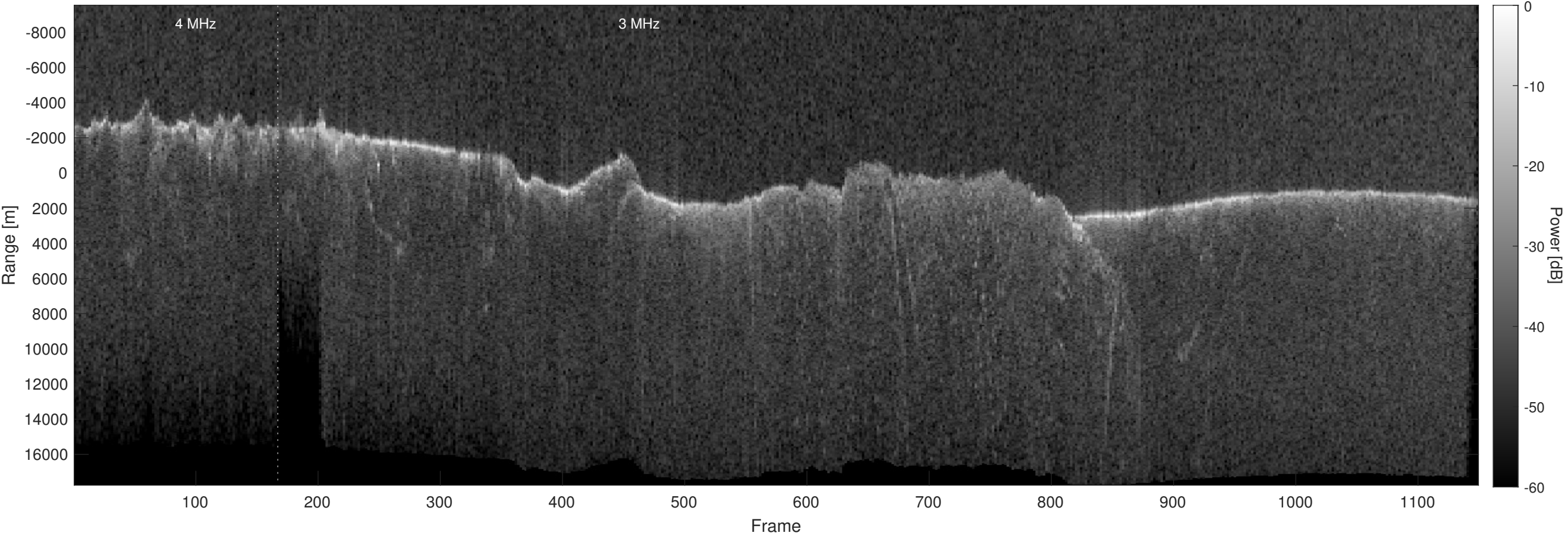
Orbit 16505, Optimized, Window, Depth-Corrected, Channel 2
