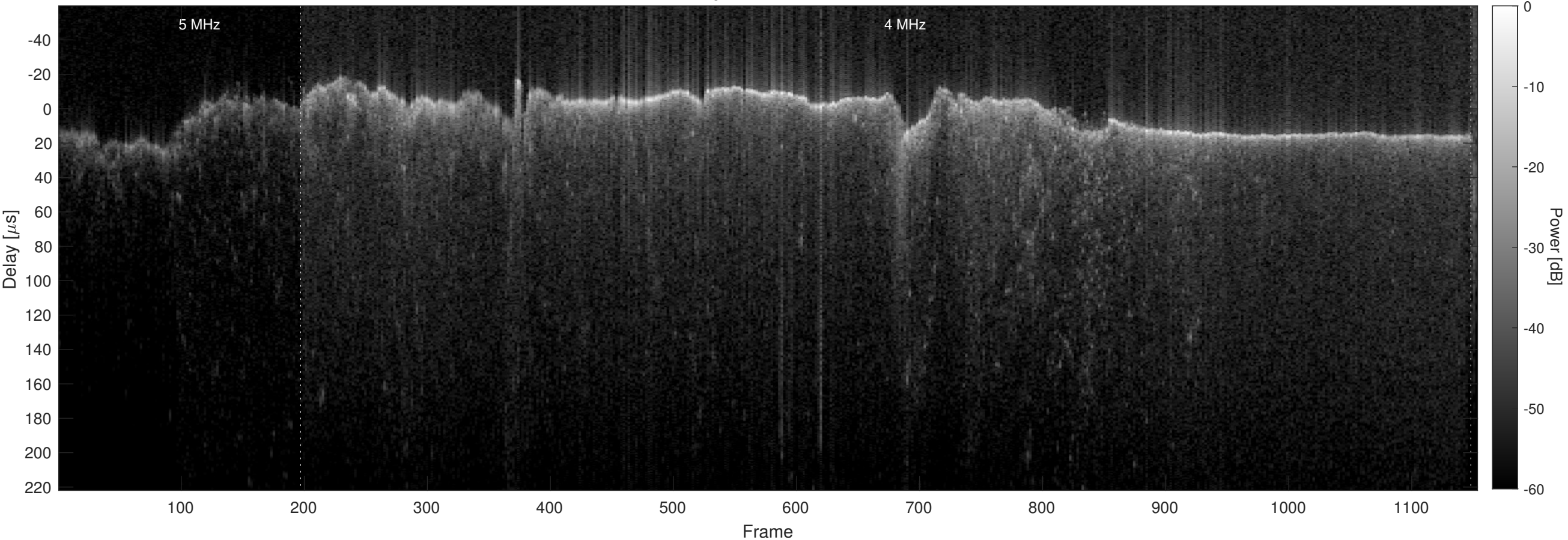
Orbit 16510, Chapman, No Window, Channel 2
