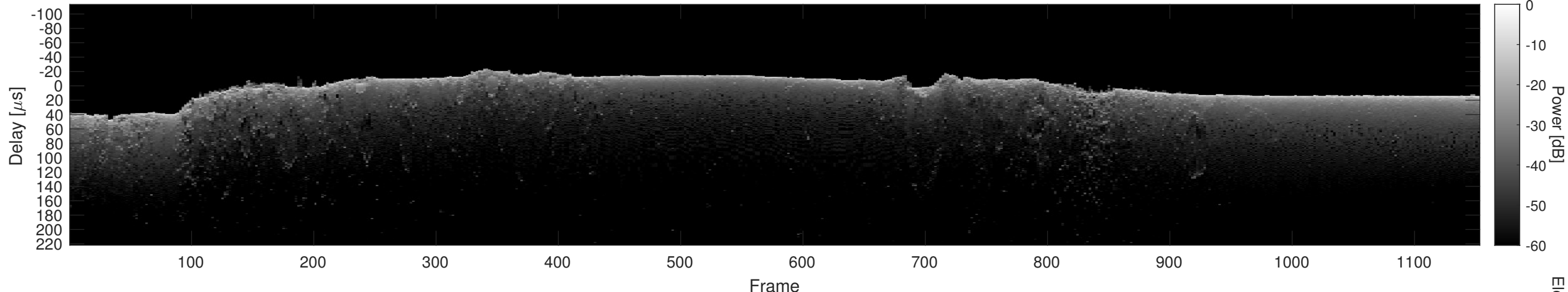
Orbit 16510, Cluttergram
