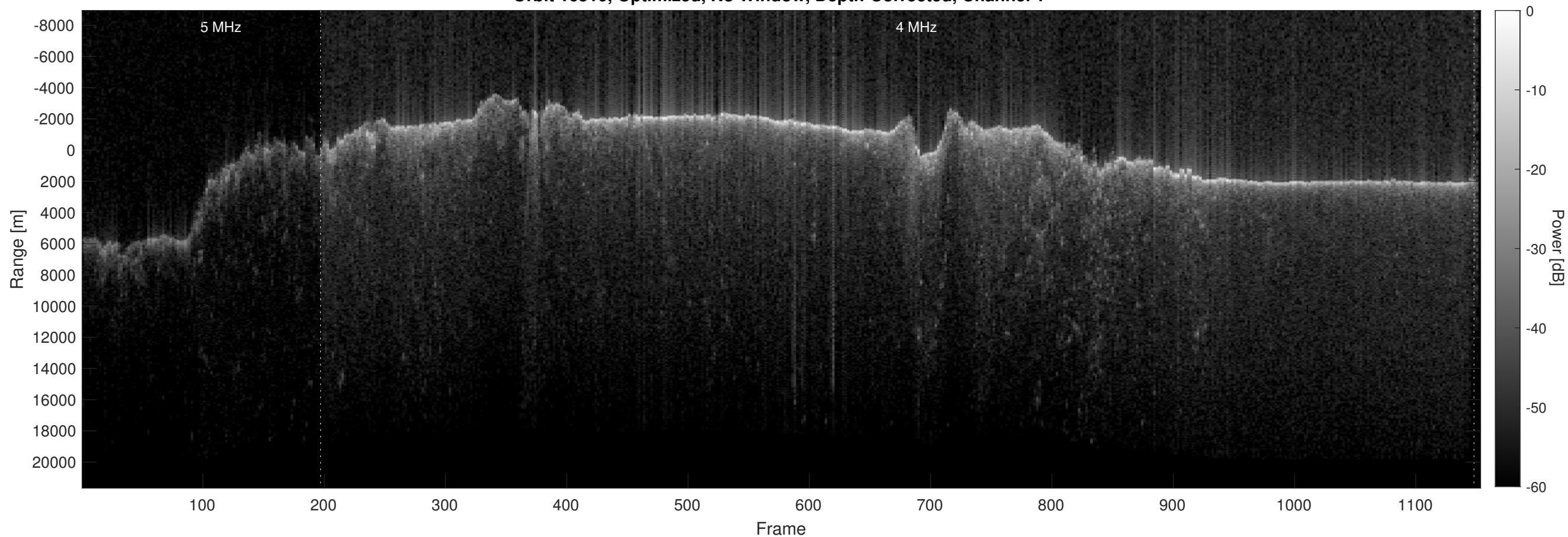
Orbit 16510, Optimized, No Window, Depth-Corrected, Channel 2
