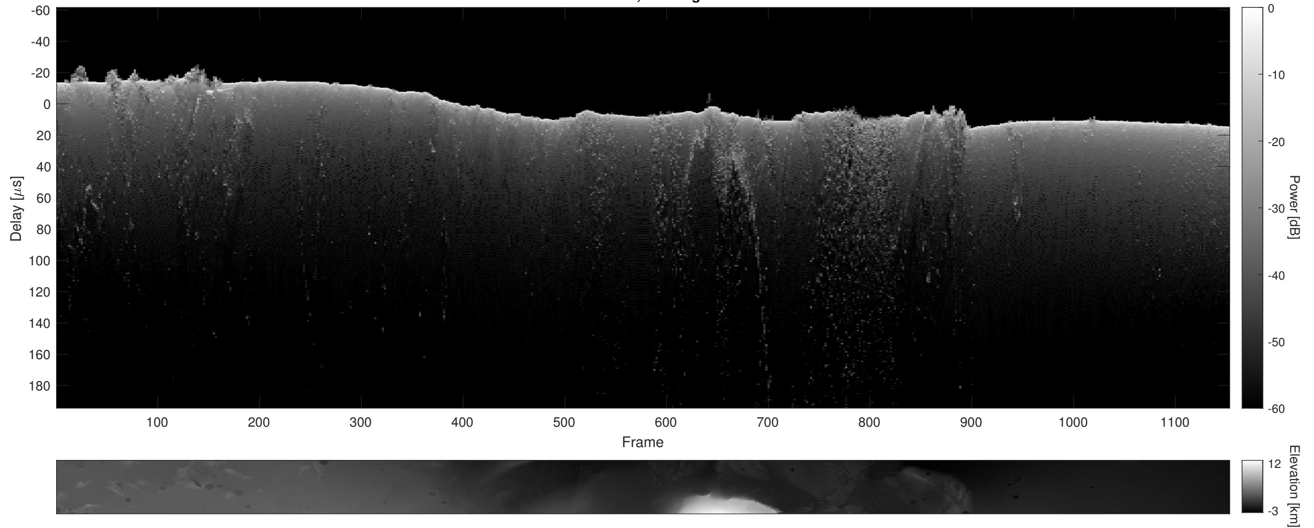
Orbit 16512, Cluttergram
