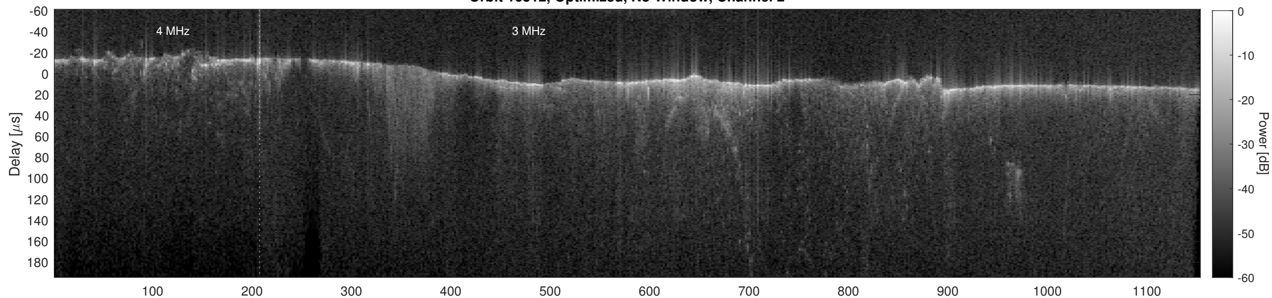
Orbit 16512, Cluttergram
