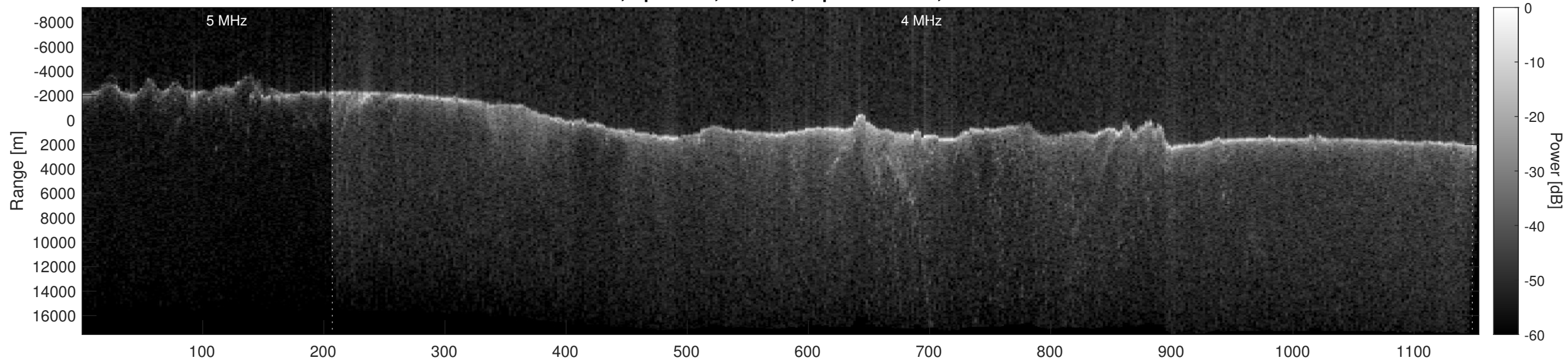
Orbit 16512, Optimized, Window, Depth-Corrected, Channel 2
