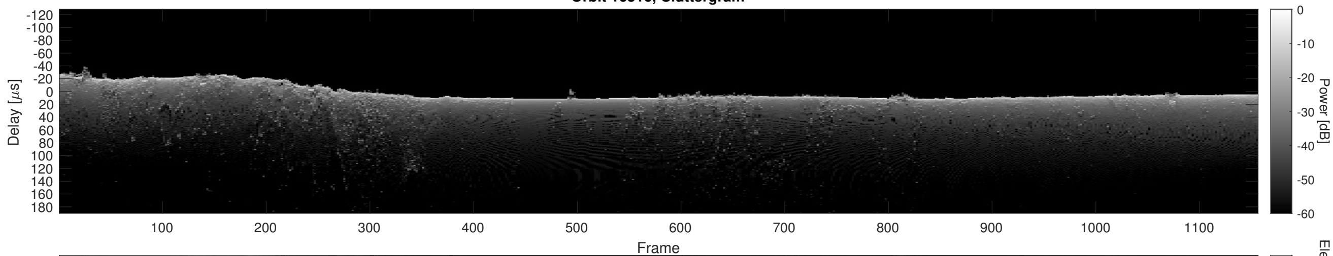
Orbit 16516, Cluttergram
