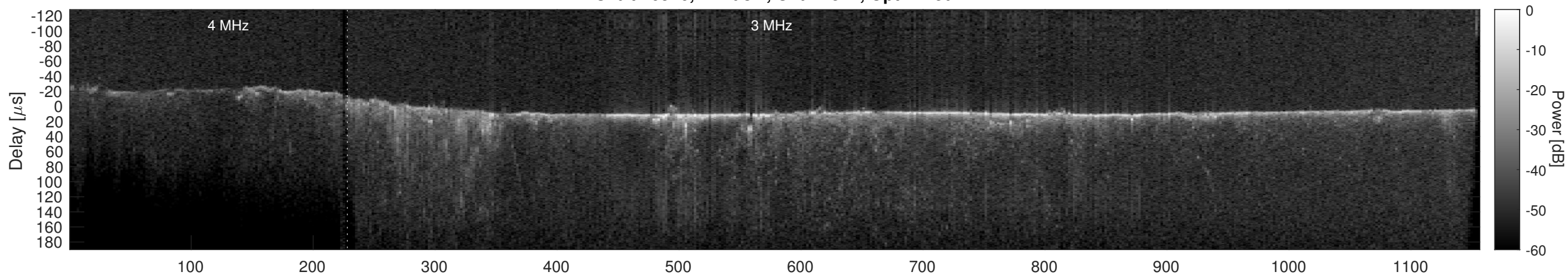
Orbit 16516, Cluttergram
