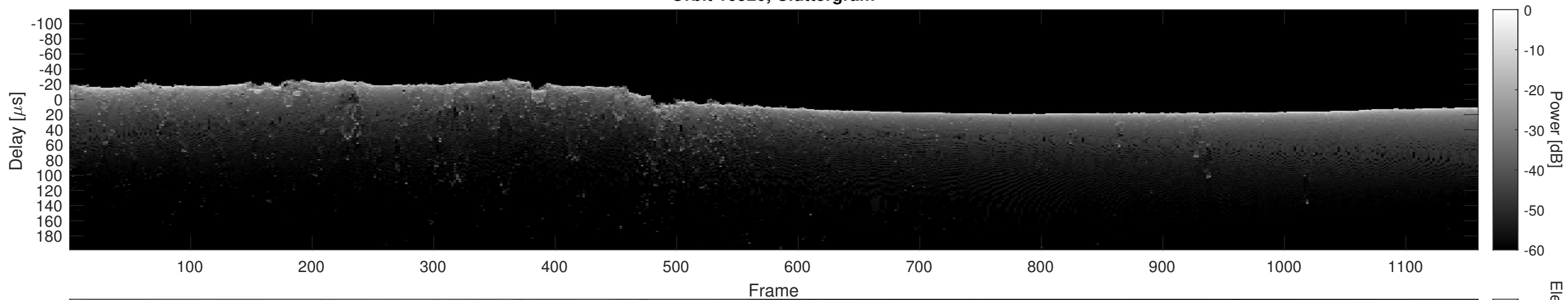
Orbit 16520, Cluttergram
