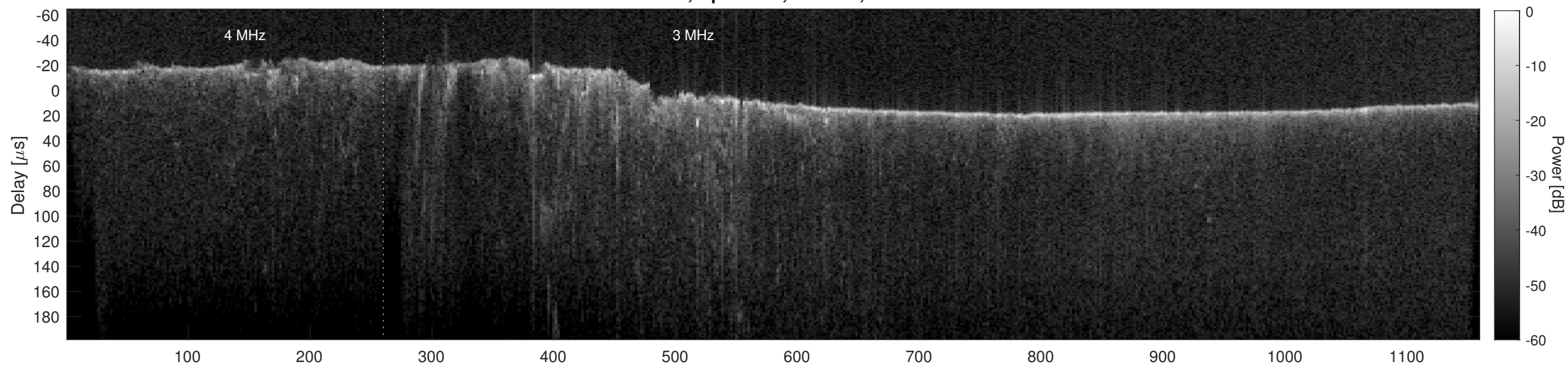
Orbit 16520, Cluttergram
