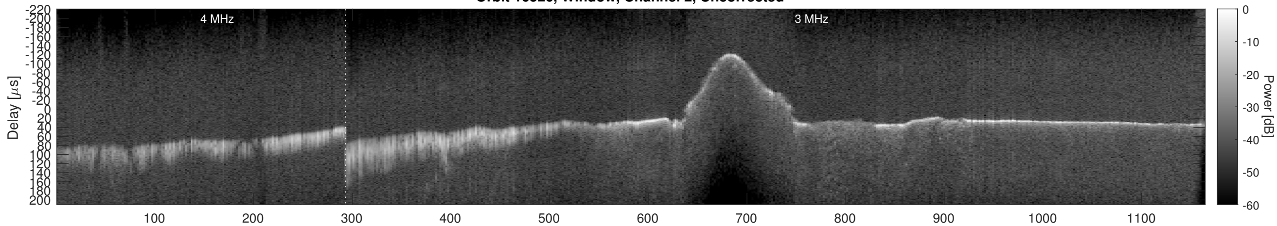
Orbit 16526, Window, Channel 2, Chapman
