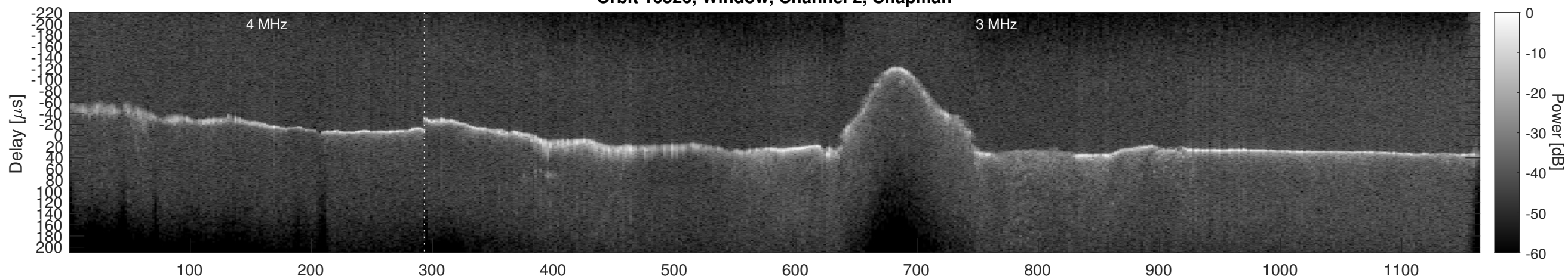
Orbit 16526, Window, Channel 2, Optimized
