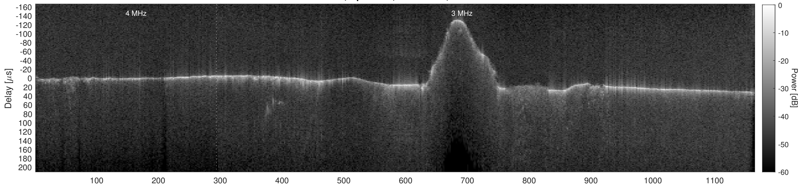
Orbit 16526, Cluttergram
