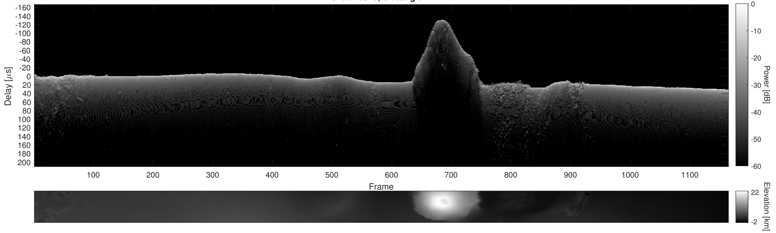
Orbit 16526, Cluttergram
