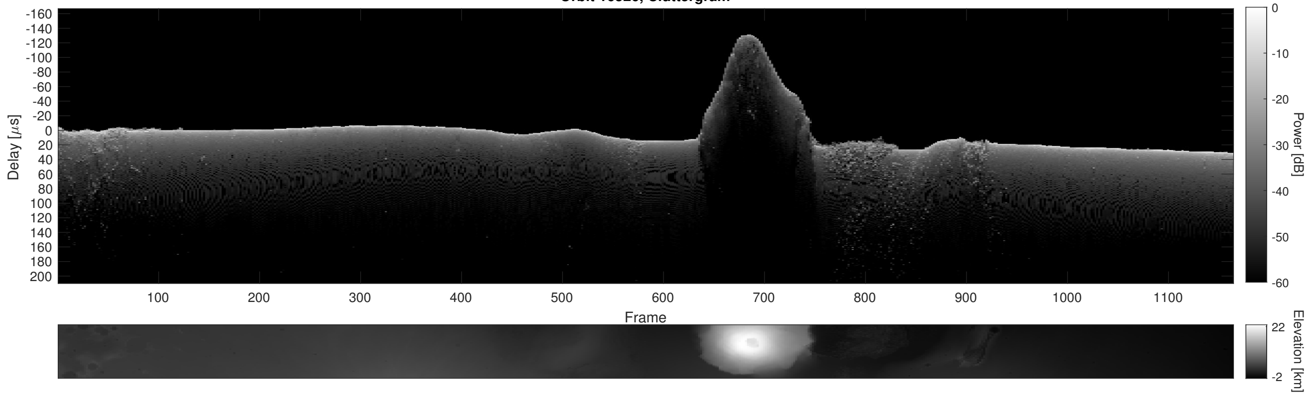
Orbit 16526, Cluttergram
