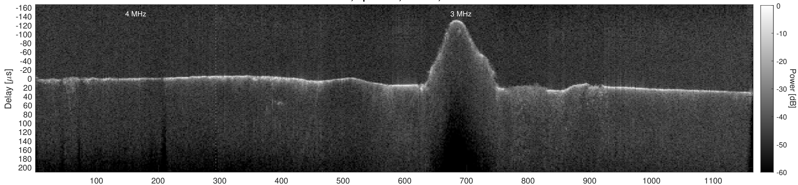
Orbit 16526, Cluttergram
