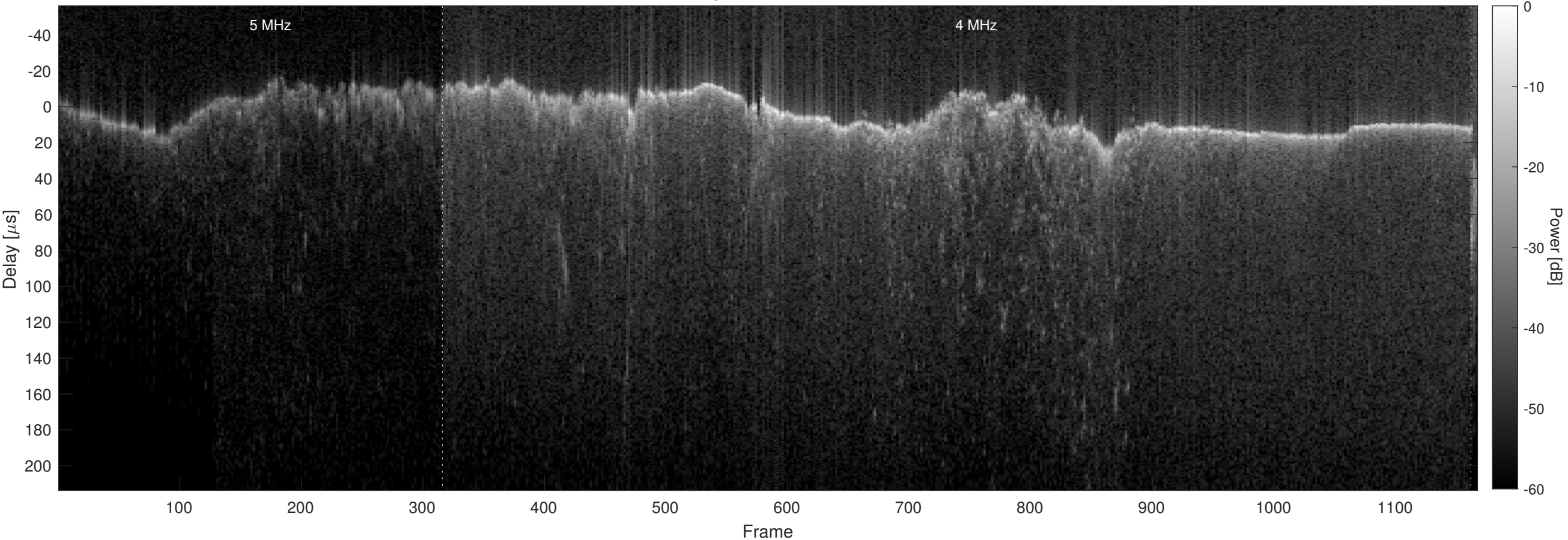
Orbit 16531, Chapman, No Window, Channel 2
