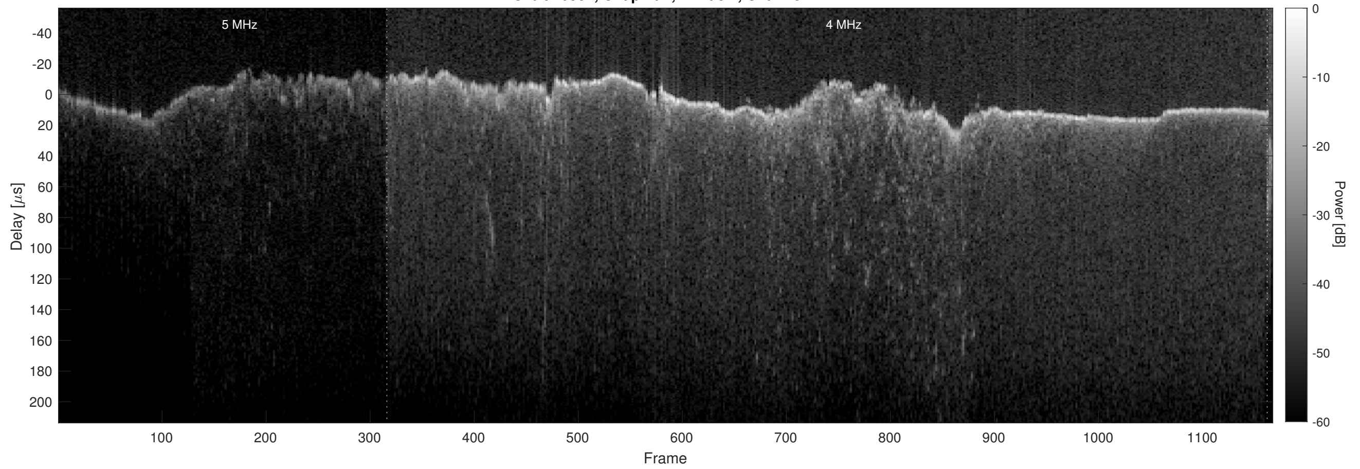
Orbit 16531, Chapman, Window, Channel 2
