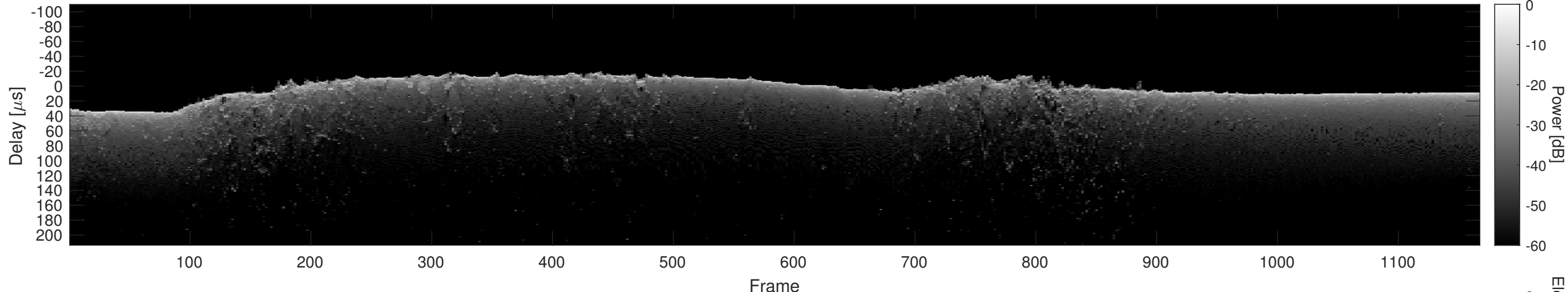
Orbit 16531, Cluttergram
