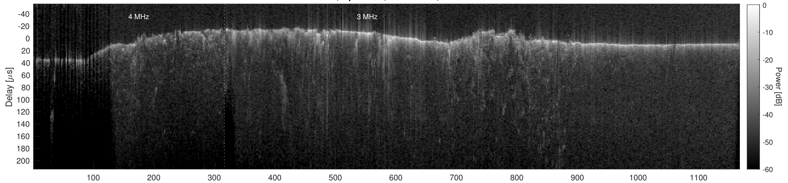
Orbit 16531, Cluttergram
