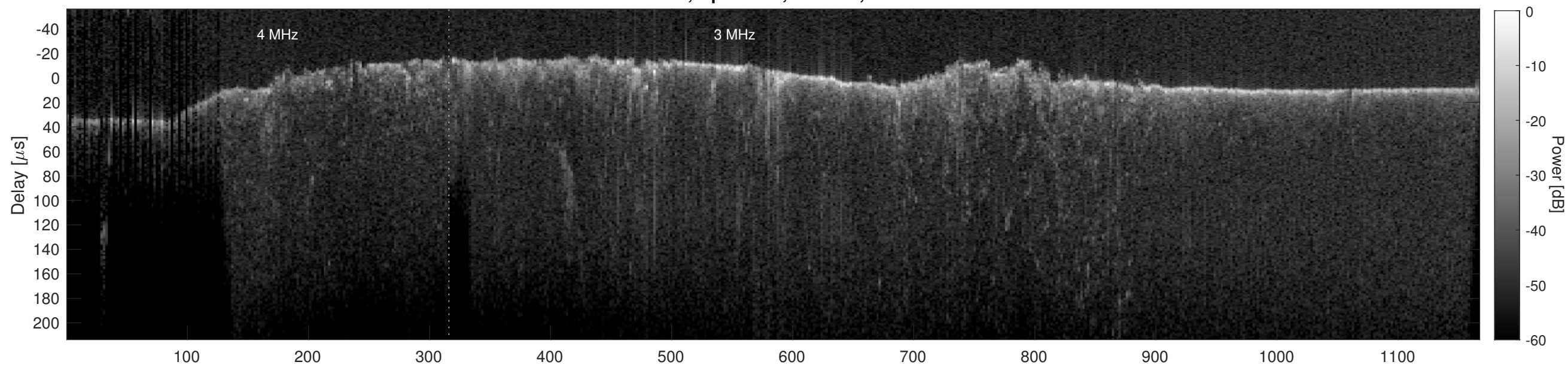
Orbit 16531, Cluttergram
