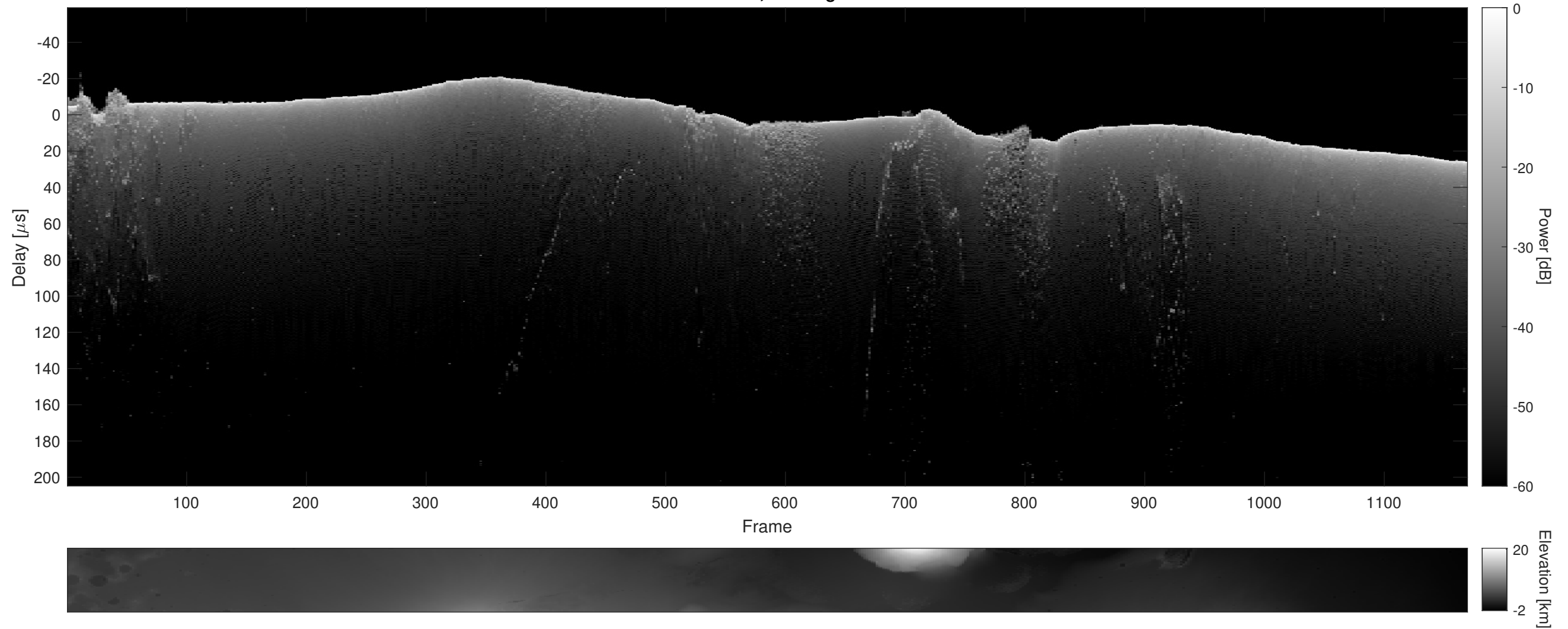
Orbit 16533, Cluttergram
