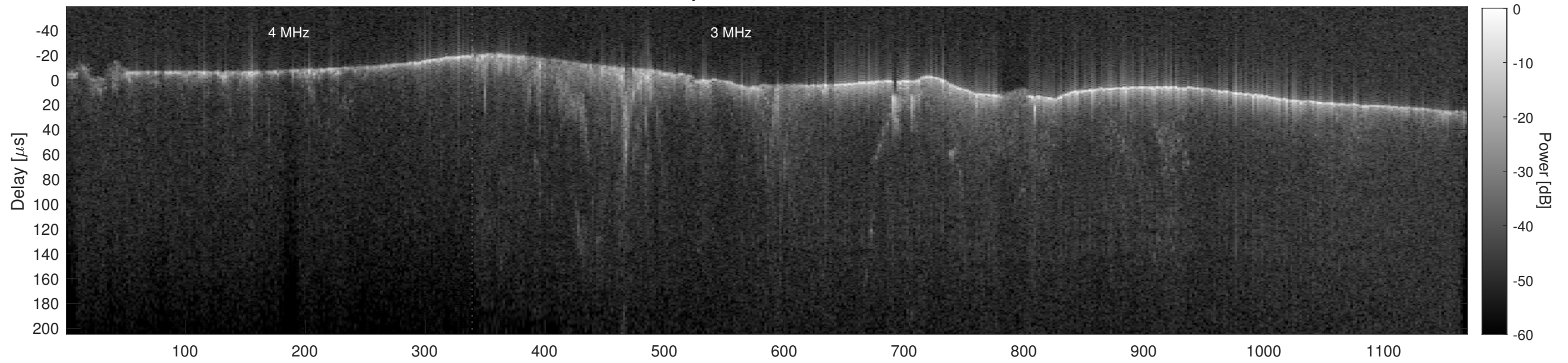
Orbit 16533, Cluttergram
