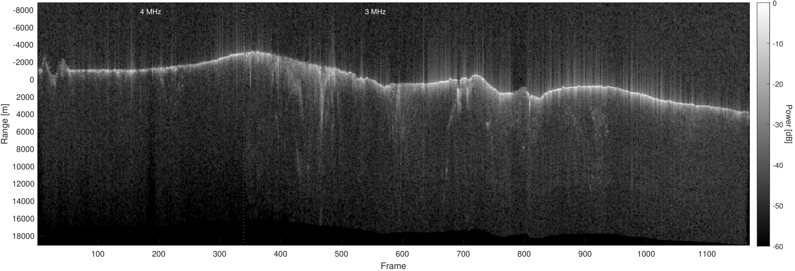
Orbit 16533, Optimized, No Window, Depth-Corrected, Channel 2
