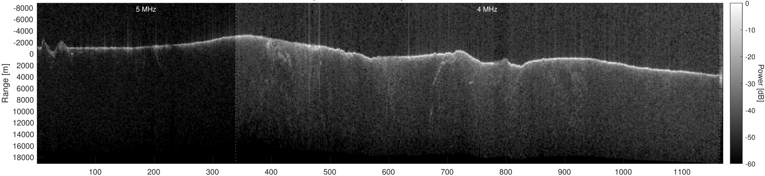
Orbit 16533, Optimized, Window, Depth-Corrected, Channel 2
