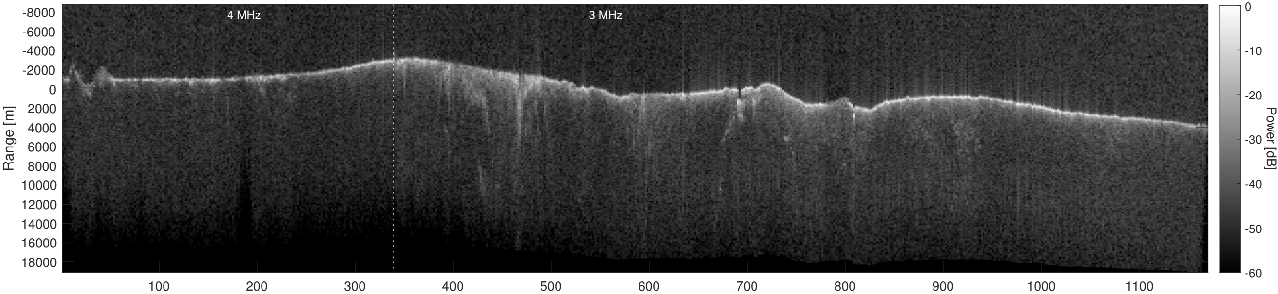
Orbit 16533, Depth-Corrected Cluttergram
