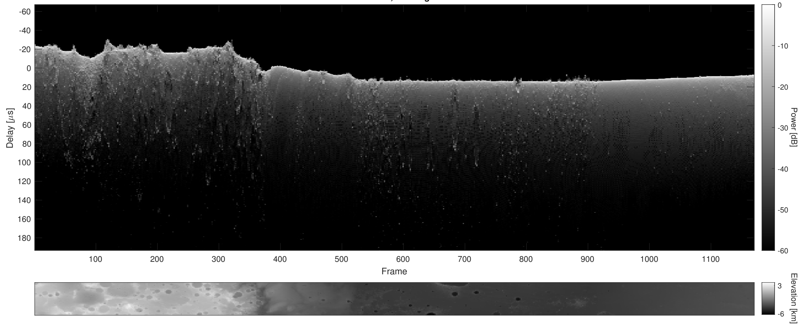
Orbit 16537, Cluttergram
