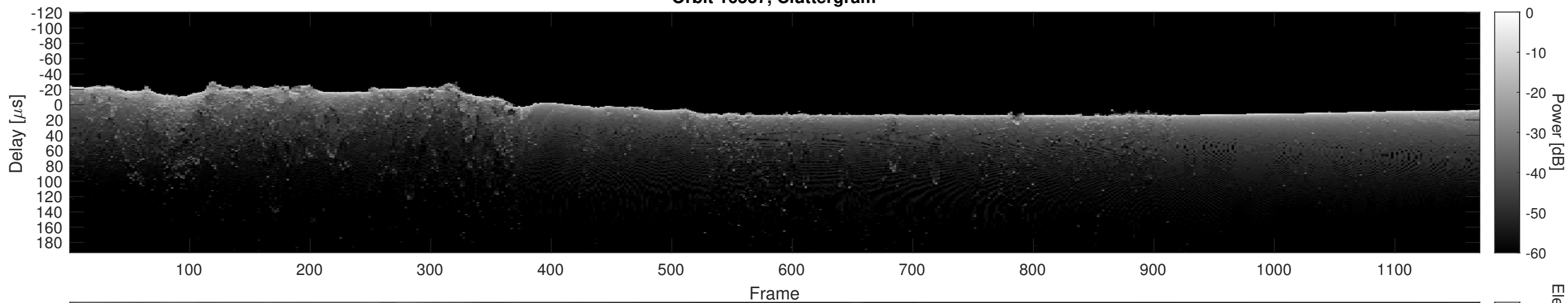
Orbit 16537, Cluttergram
