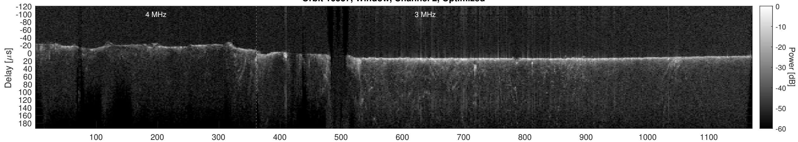
Orbit 16537, Cluttergram
