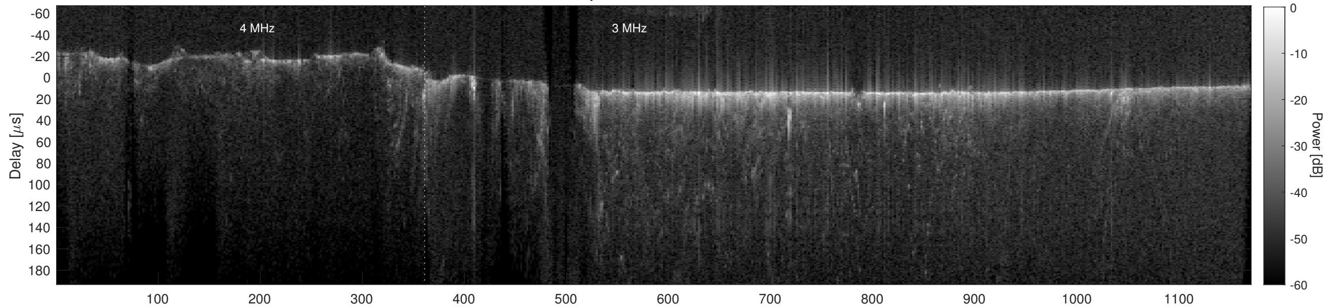
Orbit 16537, Cluttergram
