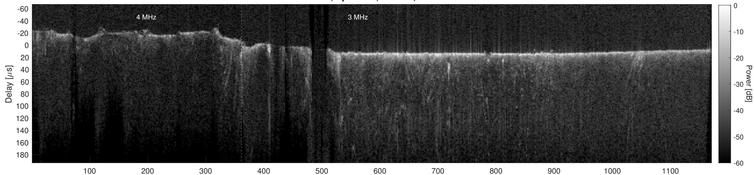
Orbit 16537, Cluttergram
