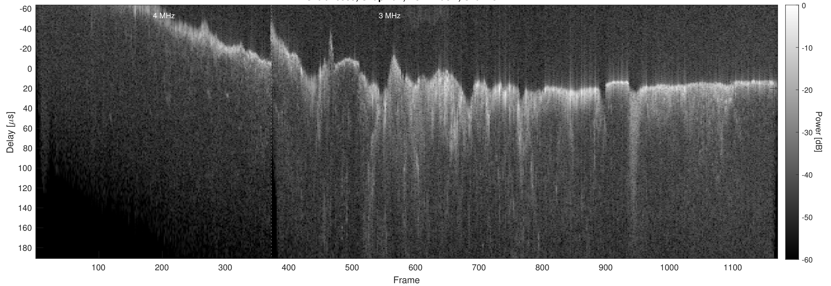
Orbit 16539, Chapman, No Window, Channel 2
