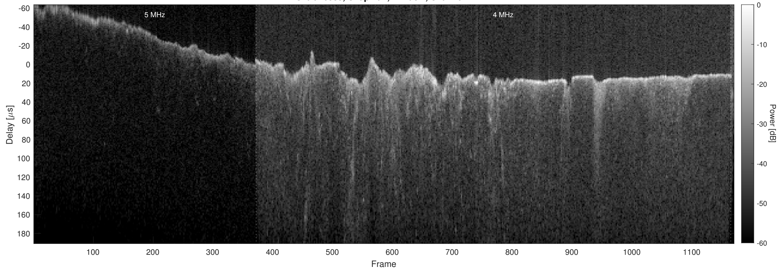
Orbit 16539, Chapman, Window, Channel 2
