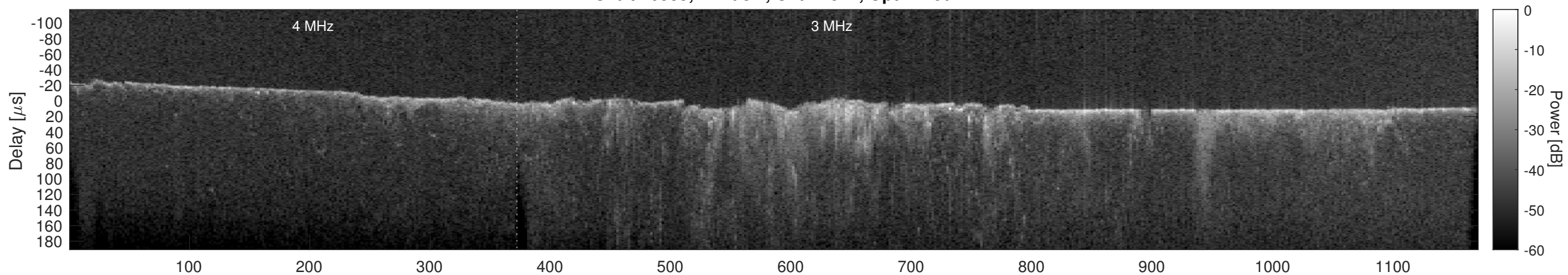
Orbit 16539, Cluttergram
