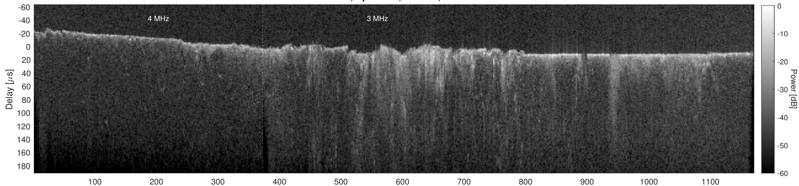
Orbit 16539, Cluttergram
