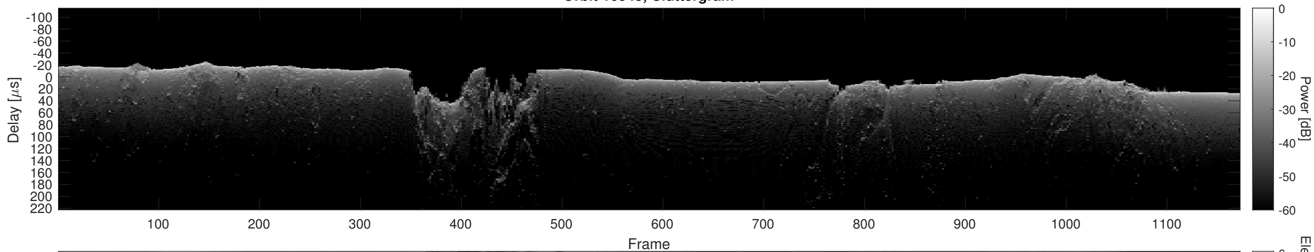
Orbit 16543, Cluttergram
