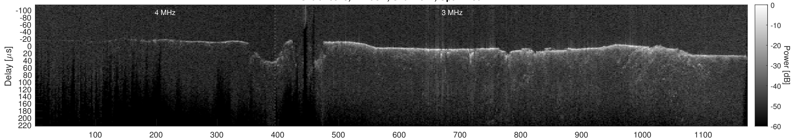
Orbit 16543, Cluttergram
