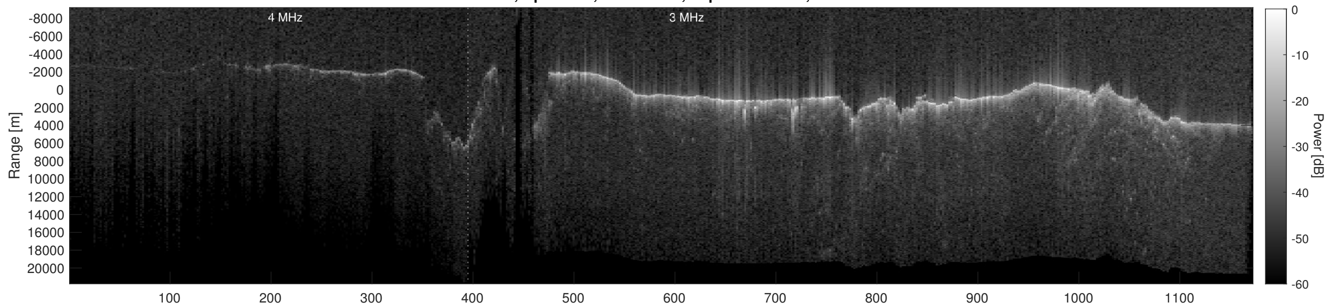
Orbit 16543, Depth-Corrected Cluttergram
