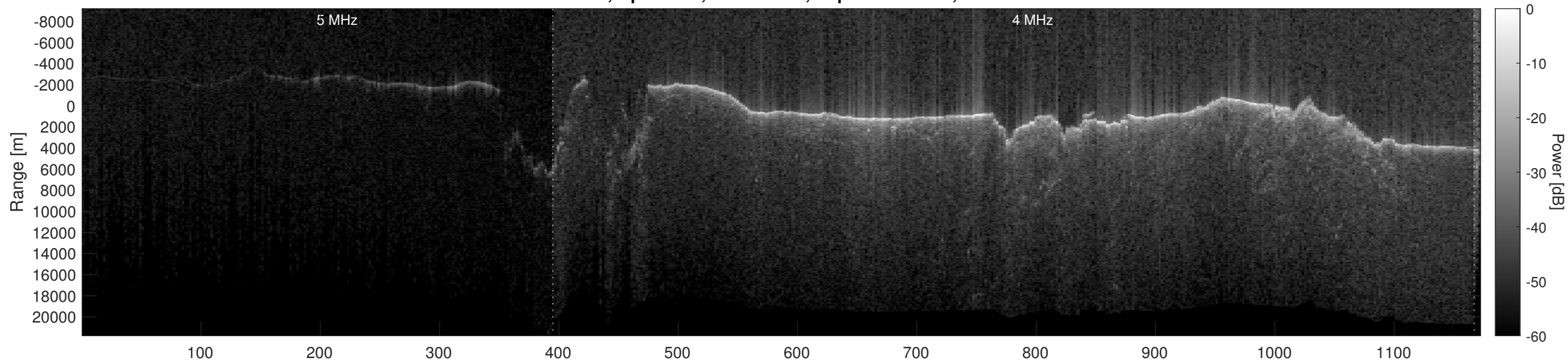
Orbit 16543, Optimized, No Window, Depth-Corrected, Channel 2
