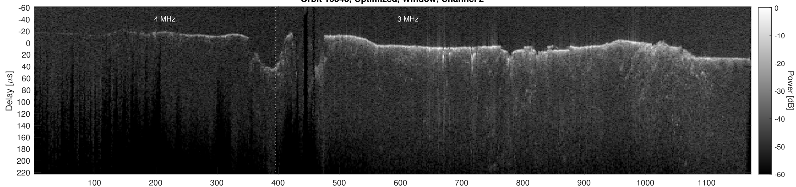
Orbit 16543, Cluttergram
