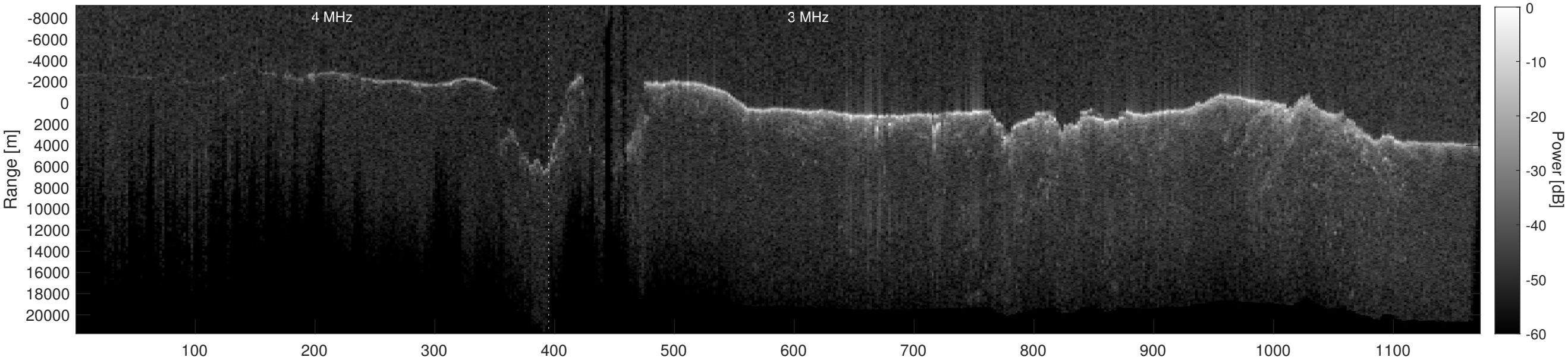
Orbit 16543, Depth-Corrected Cluttergram
