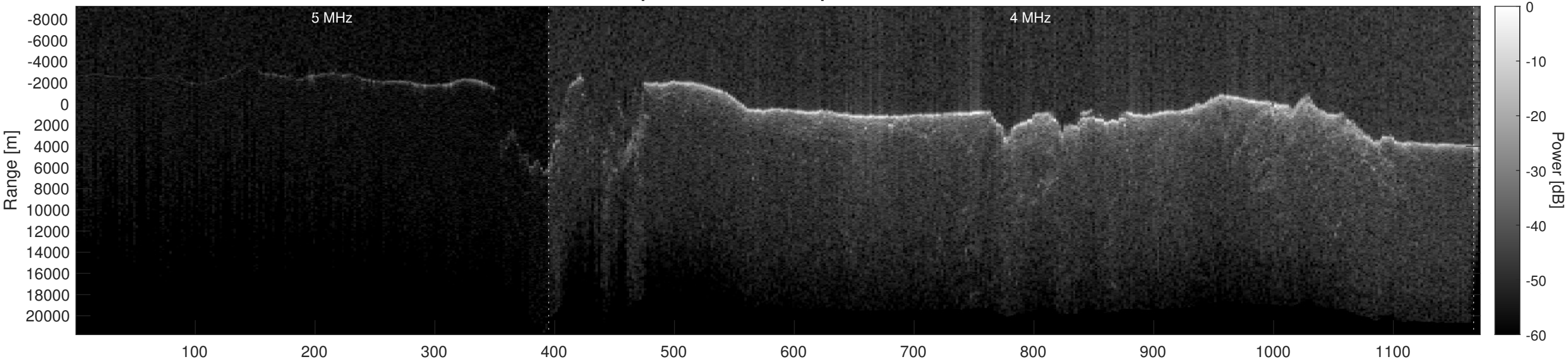
Orbit 16543, Optimized, Window, Depth-Corrected, Channel 2
