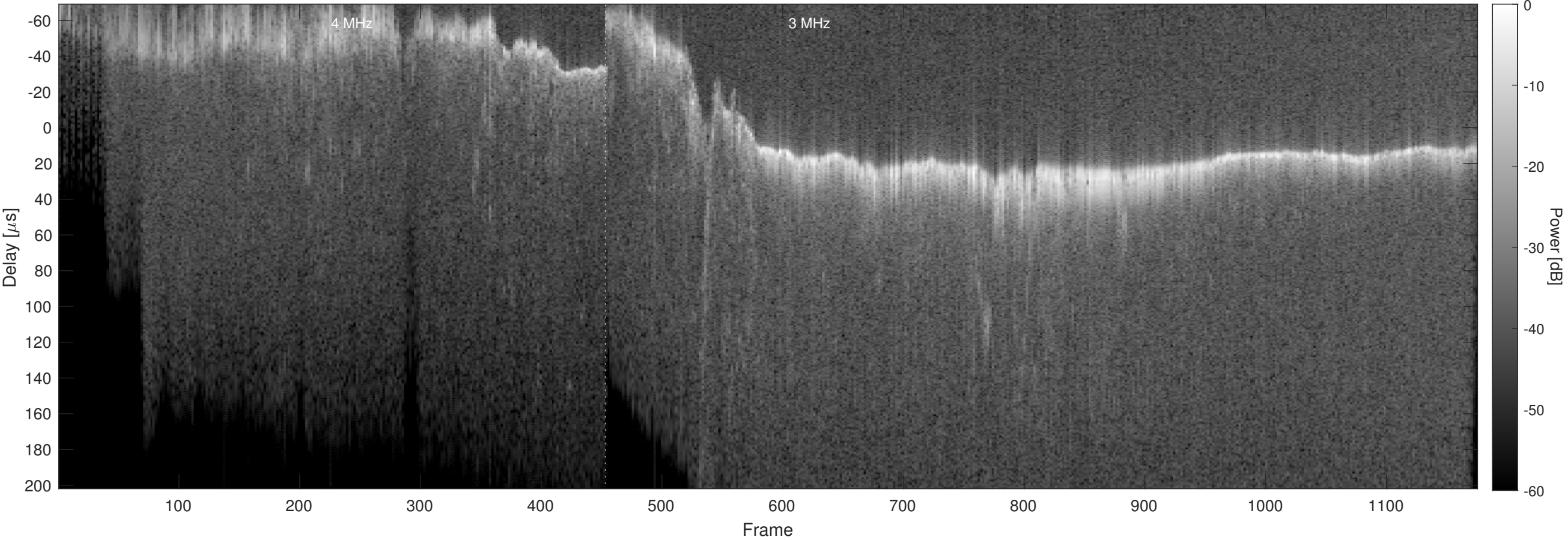
Orbit 16552, Chapman, No Window, Channel 2
