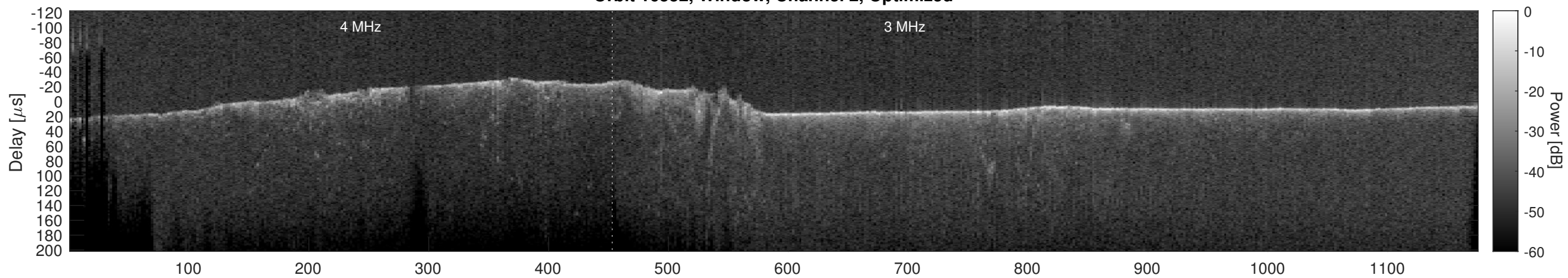
Orbit 16552, Cluttergram
